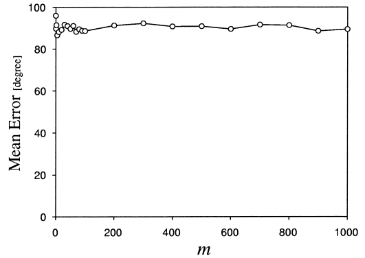
図4 BP モデルの汎化誤差とサンプル数の関係 Fig. 4 Relationship between generalization error and sample size for the BP model.
