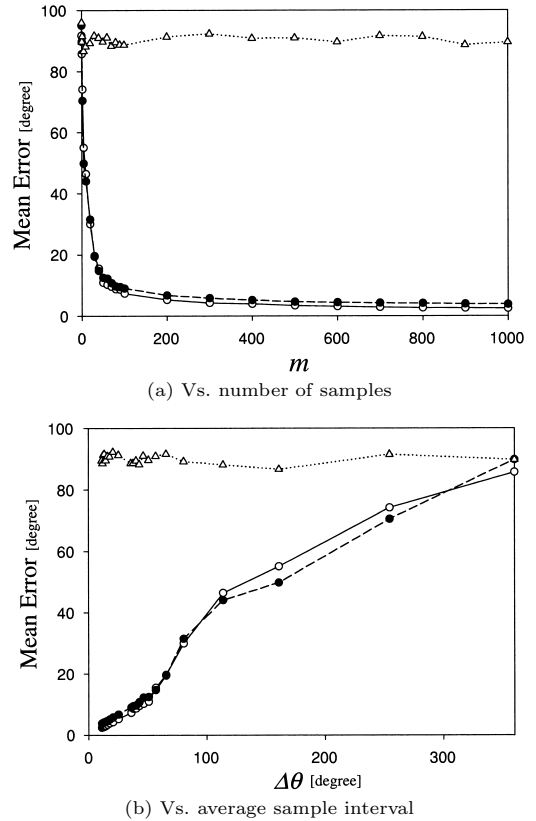
図 9 汎化誤差とサンプルサイズの関係 Fig. 9 Relationship between generalization error and sample size.
