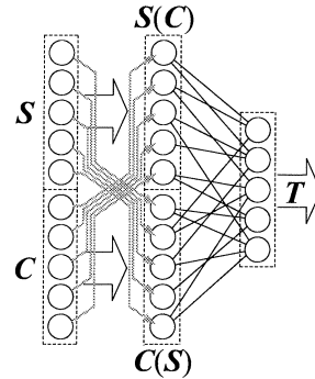
(b) Mutual modification model
